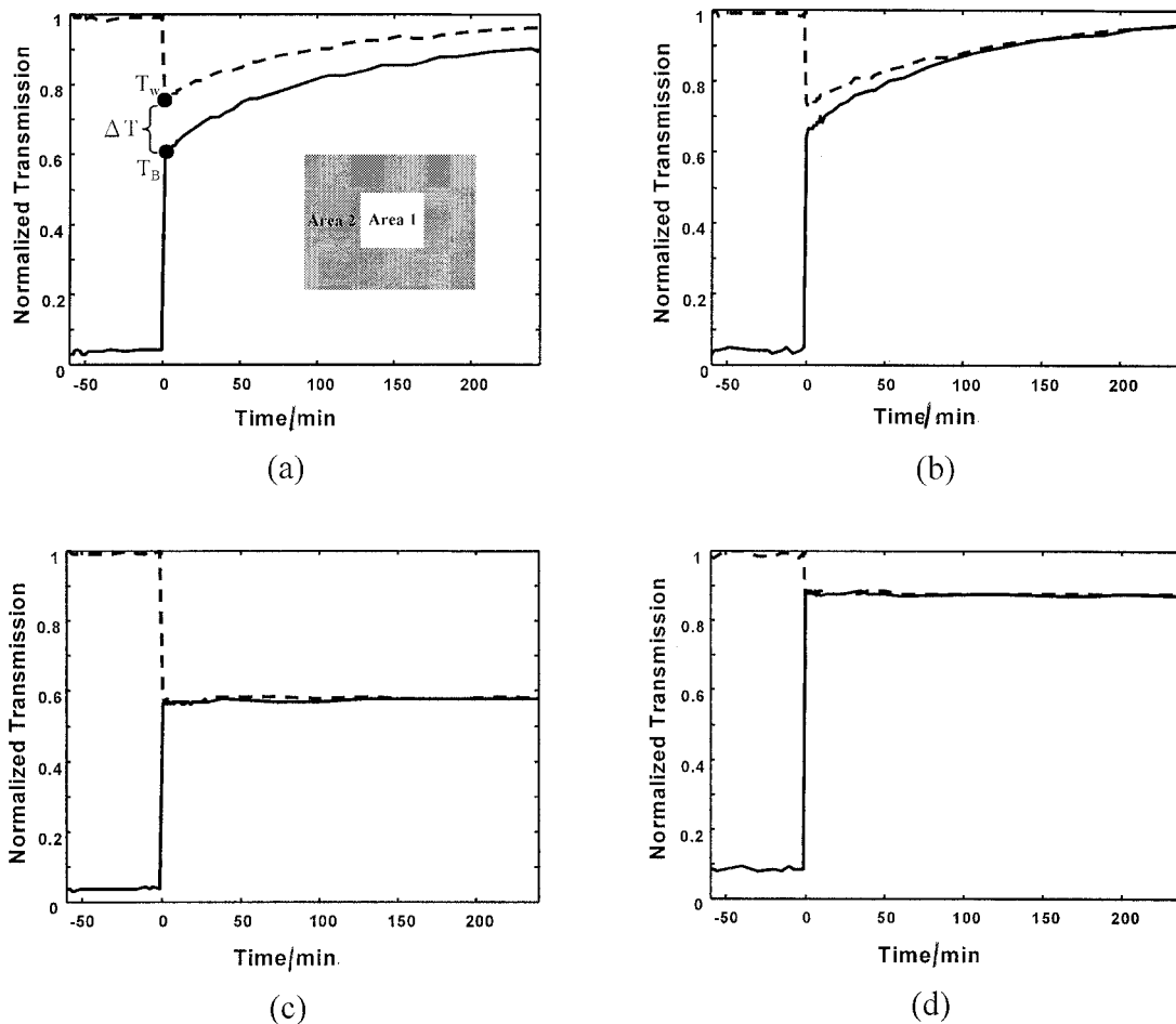
Figure 4. The T-t curves for modules 1 (a), 2 (b), 3 (c) and 4 (d) stressed for 60 min under an ambient temperature of 60^\circ\text{C} . The time at t = 0 represents the moment when pattern 1 is switched to pattern 2. Lines and \Delta T as for figure 2.
